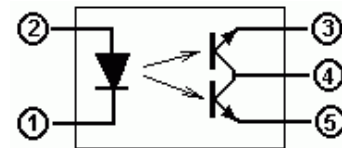
Internal Circuit
